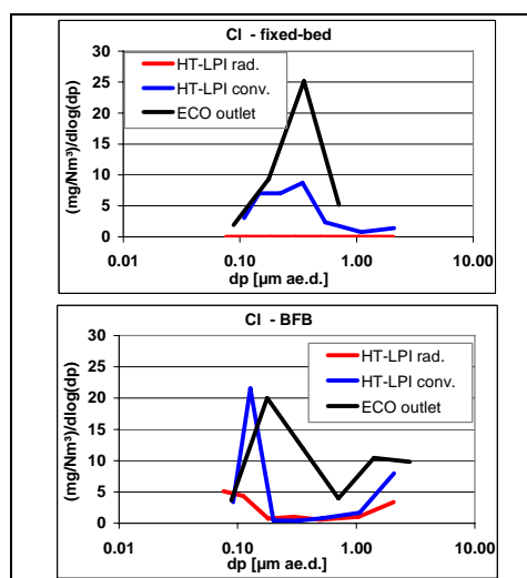
Figure 17: Concentrations of particle bound Cl in the flue gas in the radiative and the convective section as well as at boiler outlet in the fixed-bed combustion system and the BFB combustion system
