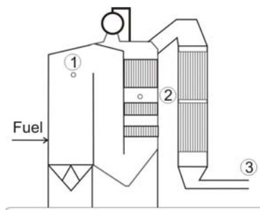
Figure 4: Scheme of the bubbling fluidised-bed waste wood combustion plant investigated
