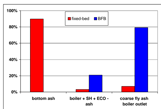
Figure 4: Ratio of the bottom ash, the boiler+SH+ECO ash and the coarse fly ash at the boiler outlet in the total ash mass flow in the fixed-bed and the BFB combustion system investigated
