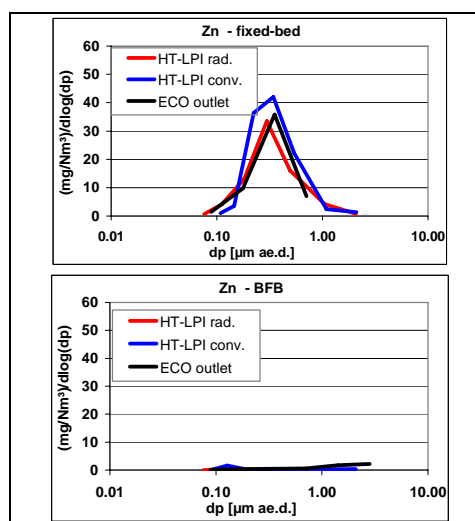
Figure 19: Concentrations of particle bound Zn in the flue gas in the radiative and the convective section as well as at boiler outlet in the fixed-bed combustion system and the BFB combustion system
