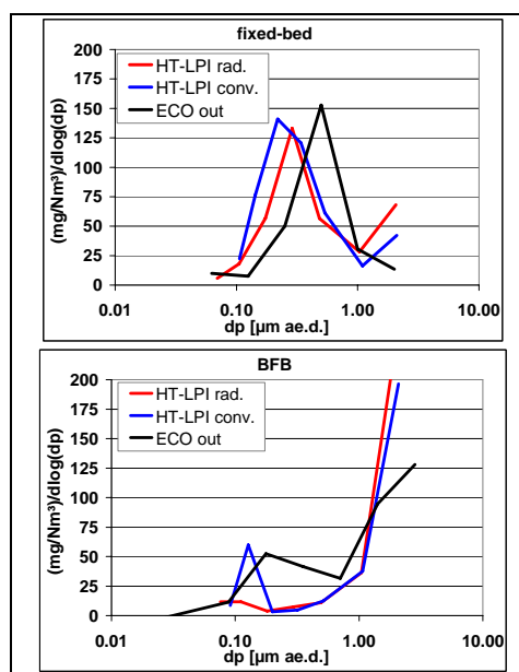
Figure 13: PSD of the aerosols in the flue gas in the radiative and the convective section as well as at boiler outlet in the fixed-bed combustion system and the BFB combustion system
