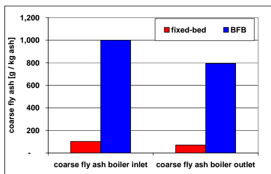
Figure 6: Trend of coarse fly ash concentration at the boiler inlet and the boiler outlet in the fixed-bed and the BFB combustion systems investigated related to ash mass flow
