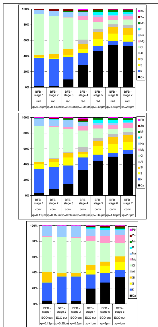
Figure 12: Chemical composition of the aerosols sampled with the HT-LPI (stages 1 to 7) as well as the BLPI (stages 1 to 6) at the waste wood fired BFB combustion plant
