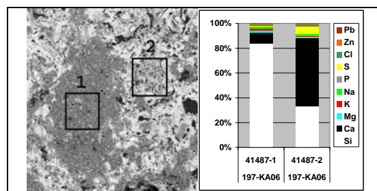
Figure 21: SEM/EDX analyses of a furnace fly ash particle (SiO 2 ) and the agglomeration (especially Ca and S) deposited in the boiler
