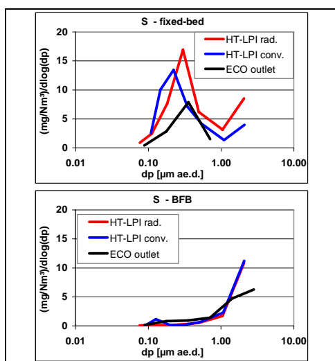
Figure 18: Concentrations of particle bound S in the flue gas in the radiative and the convective section as well as at boiler outlet in the fixed-bed combustion system and the BFB combustion system
