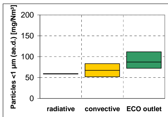
Figure 9: Aerosol concentrations in the radiative and the convective path as well as at boiler outlet in the fixed-bed combustion plant
