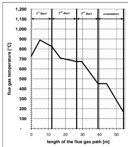
Figure 8: Trend of the flue gas temperature in the BFB combustion plant investigated from the 1 st duct to the boiler outlet
