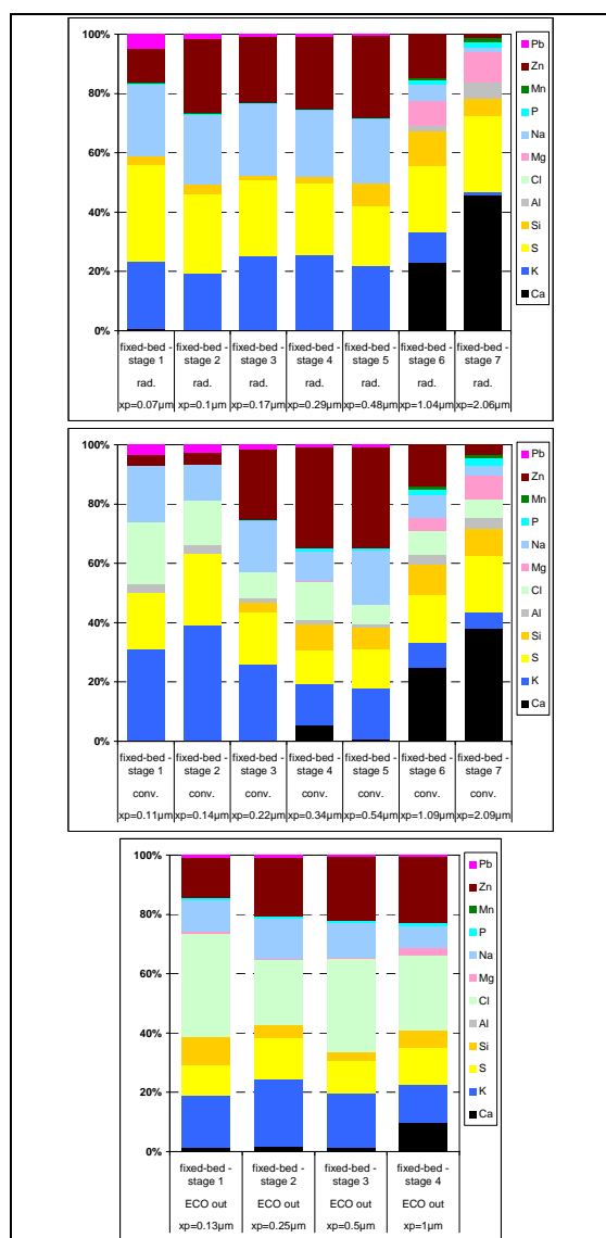
Figure 11: Chemical composition of the aerosols sampled with the HT-LPI (stages 1 to 7) as well as the BLPI (stages 1 to 4) at the waste wood fired fixed-bed combustion plant
