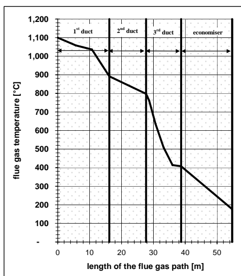
Figure 7: Trend of the flue gas temperature in the fixed-bed combustion plant investigated from the 1 st duct to the boiler outlet
