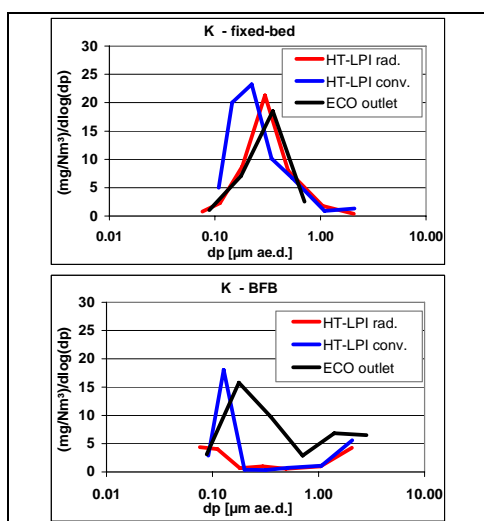
Figure 14: Concentrations of particle bound K in the flue gas in the radiative and the convective section as well as at boiler outlet in the fixed-bed combustion system and the BFB combustion system
