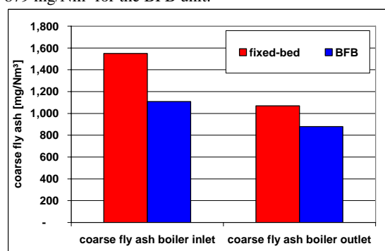
Figure 5: Trend of coarse fly ash concentrations at the boiler inlet and the boiler outlet in the waste wood fired fixed-bed and the BFB combustion plants investigated
