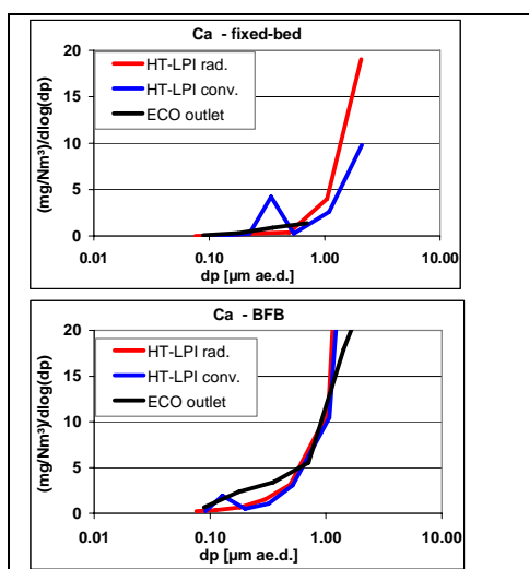
Figure 16: Concentrations of particle bound Ca in the flue gas in the radiative and the convective section as well as at boiler outlet in the fixed-bed combustion system and the BFB combustion system
