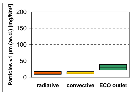
Figure 10: Aerosol concentrations in the radiative and the convective path as well as at boiler outlet in the BFB combustion plant
