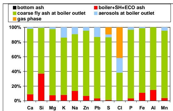
Figure 20: Involvement of elements in the ash mass fractions and the gas phase in the waste wood fired BFB combustion system
