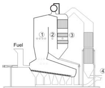
Figure 3: Scheme of the grate-fired waste wood combustion plant investigated
