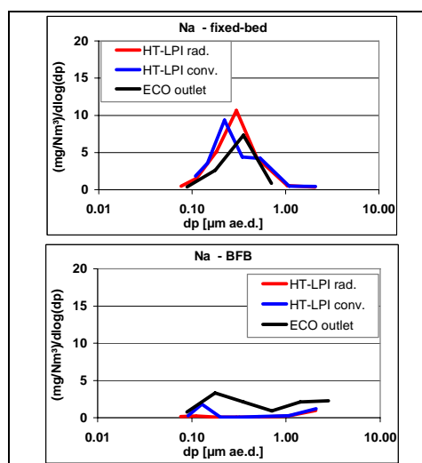
Figure 15: Concentrations of particle bound Na in the flue gas in the radiative and the convective section as well as at boiler outlet in the fixed-bed combustion system and the BFB combustion system
