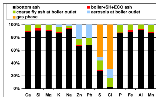
Figure 19: Involvement of elements in the ash mass fractions and the gas phase in the waste wood fired fixed-bed combustion system
